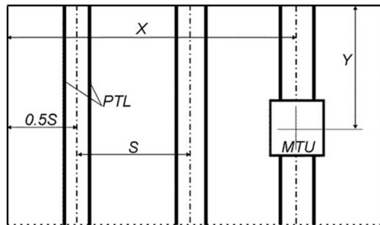
Figure 9. Diagram for determining MTU coordinates on a field with PTL.
