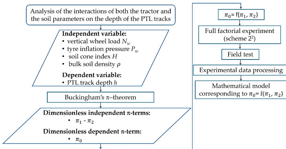
Figure 3. Research algorithm.
