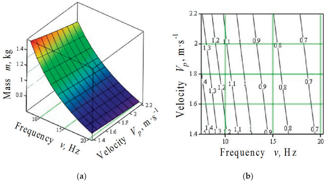
Figure 6.2. Surface (a) and contour diagrams (b) of values for digging tool mass reduced to point of impact m = (v, V_p) (kg) (digging tool running depth z = 0.10 m; oscillation amplitude a = 0.016 m).
