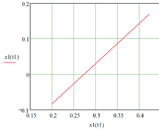
Figure 5.14. Beet root motion trajectory in the coordinate system x_1O_1z_1 during the direct lifting of the root from the soil: ( H = 500 N, P_1 = 400 N, R_x = 100 N, R_z = 100 N, \nu = 10 Hz).
