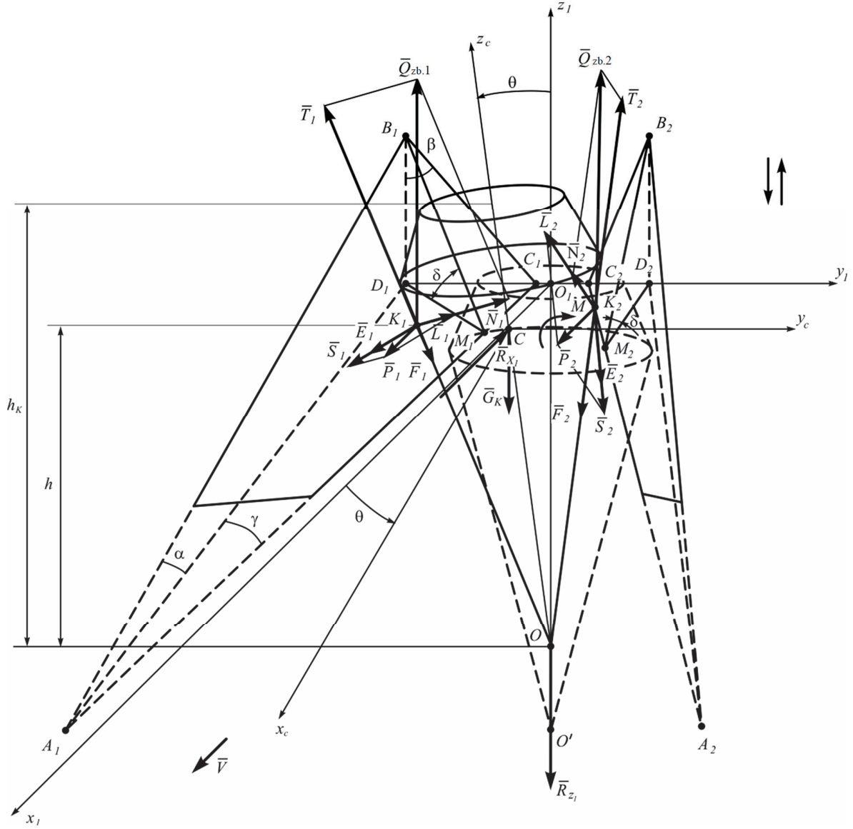
Figure 5.12. Force interaction between root and wedges of vibrating digging tool during its direct extraction from soil.
