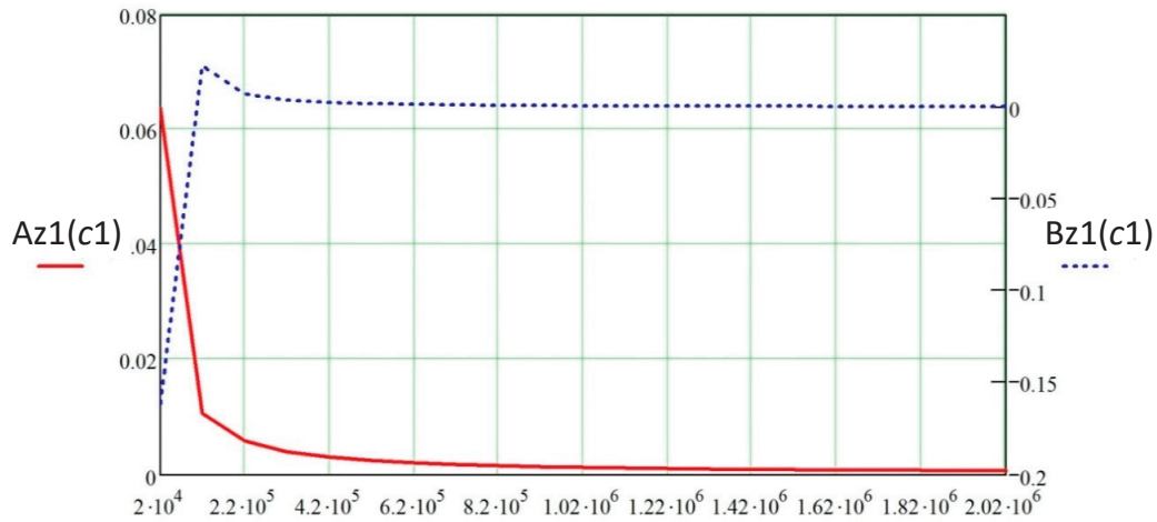
Figure 5.7. Graphs of relation between amplitudes of free A_{z1} and free accompanying oscillations B_{z1} along axis Oz_1 and soil's elastic deformation coefficient c ( H = 500 N; P_1 = 400 N; v = 10 Hz).
