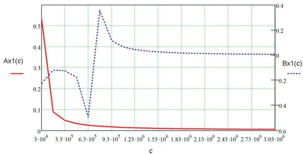
Figure 5.6. Graphs of relation between amplitudes of free A_{x1} and free accompanying oscillations B_{x1} along axis Ox_1 and soil's elastic deformation coefficient c ( H = 500 \text{ N} ; P_1 = 400 \text{ N} ; v = 10 \text{ Hz} ).
