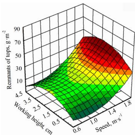
Figure 4. The response surface of haulm residues on root crowns against the speed of the cleaner and the elevation of the blades at the angular velocity of the cleaning tool's rotation of 76.8 rad s -1 .
