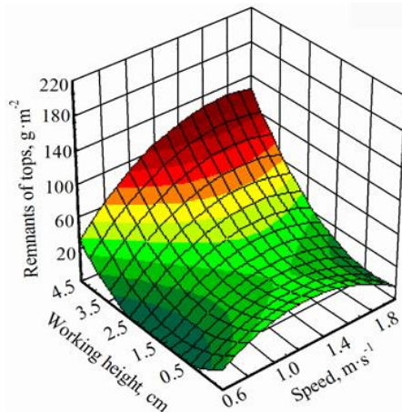
Figure 5. The response surface of haulm residues on root crowns against the speed of the cleaner and the elevation of the blades at the angular velocity of the cleaning tool's rotation of 56.5 rad s -1 .
